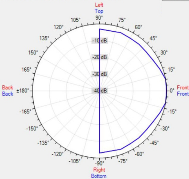
Data Shown: CM6TSMF (Apart Audio) Display Parameters: Frequency: 4000Hz (1/24th Octave)
