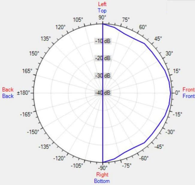
Data Shown: CM6TSMF (Apart Audio) Display Parameters: Frequency: 1000Hz (1/24th Octave)
